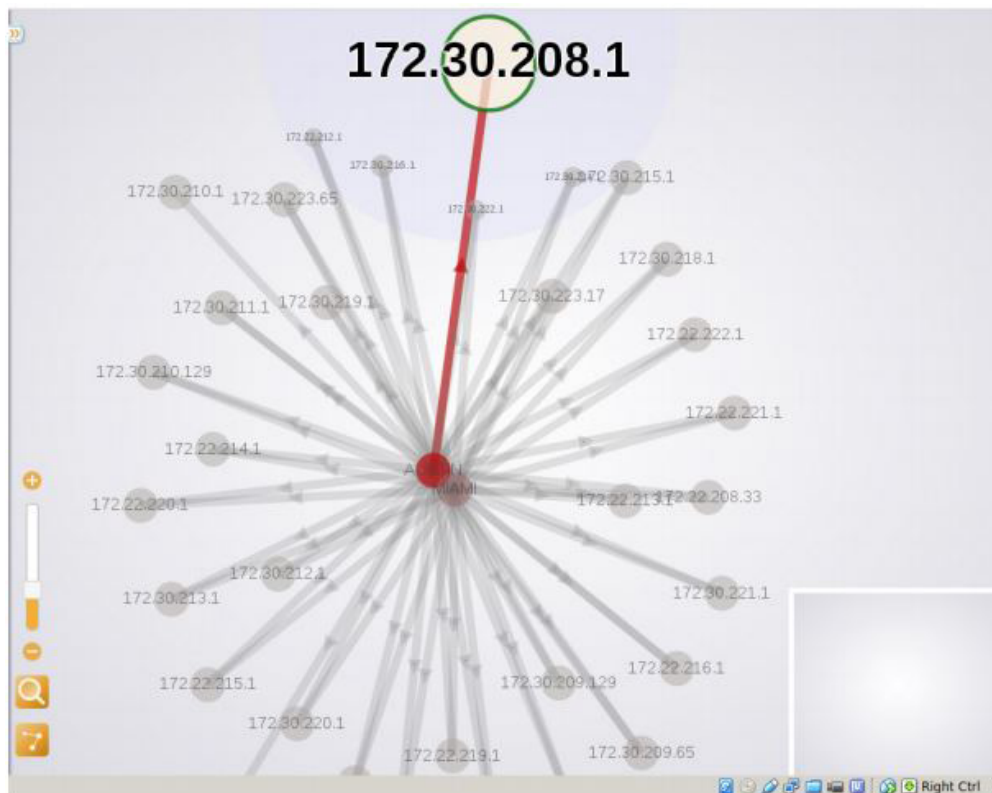
Visualization of the virtual routing redundancy protocol (VRRP) cluster in existing configurations which illustrates a misconfiguration in the cluster. Only the red router fields packets to virtual IP address 172.30.208.1; in the event of a failure of the red router, the gray router will not field packets with this virtual IP address.
